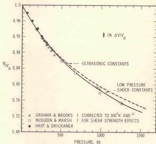
Fig. 1. High-pressure isothermal compression curves for sapphire. The dotted and solid lines are the relationships predicted by the Murnaghan equation with constants derived ultrasonically [ Gieske and Barsch , 1968] and with constants derived from the low-pressure shock data of Graham and Brooks [1971]. The shock data are corrected for thermal pressure and shear strength offsets. The static isothermal compression data of Hart and Drickamer are also shown. The extent to which the data agree with the Murnaghan relations provides a direct measure of the adequacy of the linear bulk modulus approximation for sapphire. The agreement between all experimental points and the isothermal compression curve is thought to be within the experimental error of the measurements.
